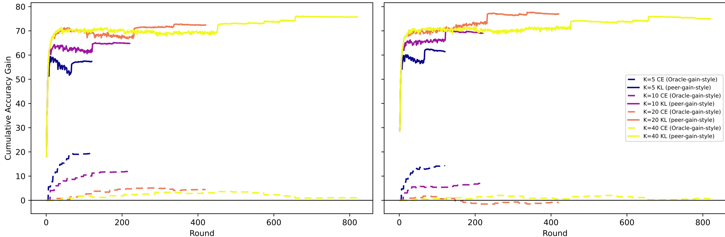
CE-pretrained teacher
